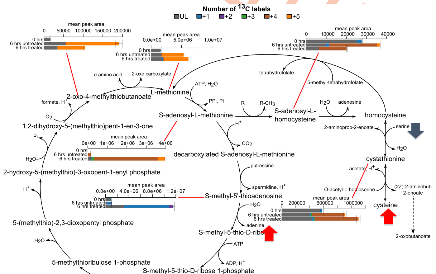
Fig 4. Tracing 13 C distribution in AN5568-treated cells incubated with 13 C-U-L-methionine. Cells were incubated with 200 μM [U- 13 C]-L-methionine for 6 hours. In addition, one sample group was incubated with 1.9 μM (10× EC 50 ) AN5568. Metabolites involved in L-methionine metabolism detected in this experiment were overlaid onto metabolic maps. In cases where 13 C isotopes were detected, graphs incorporating the percentage labelling are shown. The methionine salvage pathway (Yang cycle) is shown.
